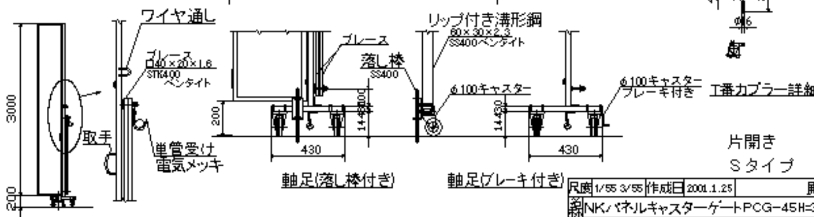
A 矢視 (A view)
